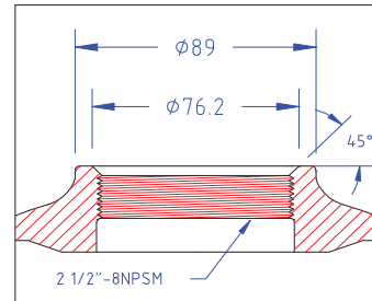
DETAIL 2 1/2" THREAD
